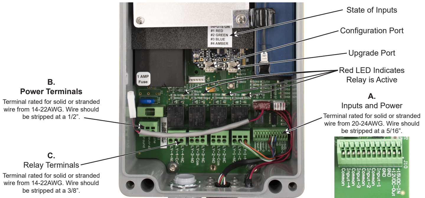
Inside View of MS2000X with -AC, -B, and -LS Options Installed
